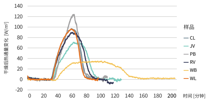
图6 6种纺织面料的热通量分布 (CL - 亲水性棉布, JV - 疏水性粘胶单面针织物, PB - 亲水性涤纶罗纹, RV - 疏水性粘胶罗纹, WB - 疏水性羊毛针织物, WL - 亲水性羊毛针织物)
